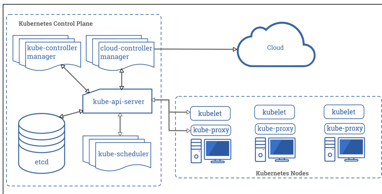
Figure 2: Kubernetes architecture 1
