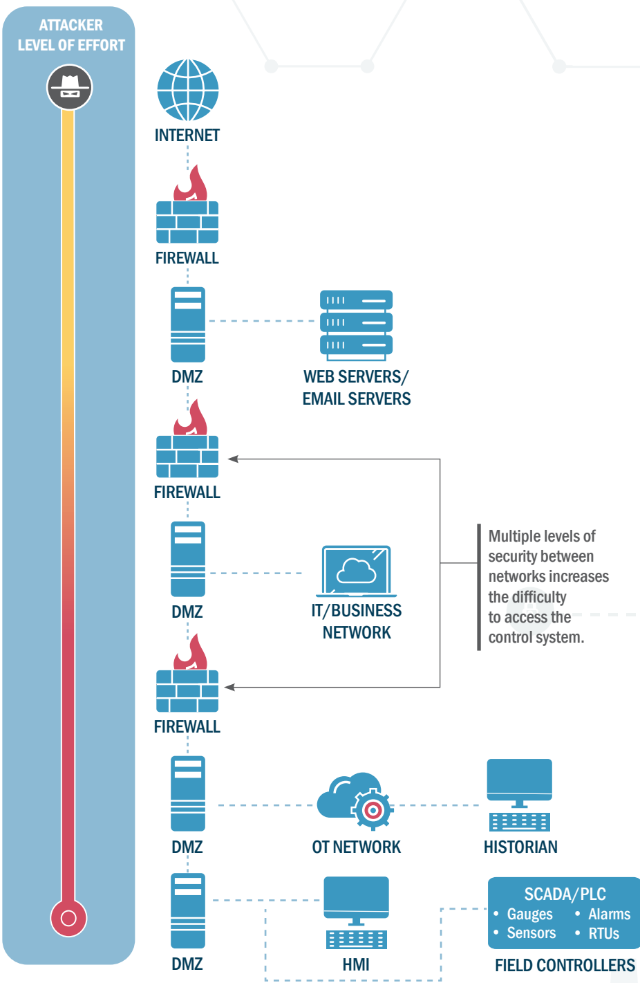
FIGURE 2: A SEGMENTED PURDUE ENTERPRISE REFERENCE ARCHITECTURE (PERA) NETWORK ARCHITECTURE
